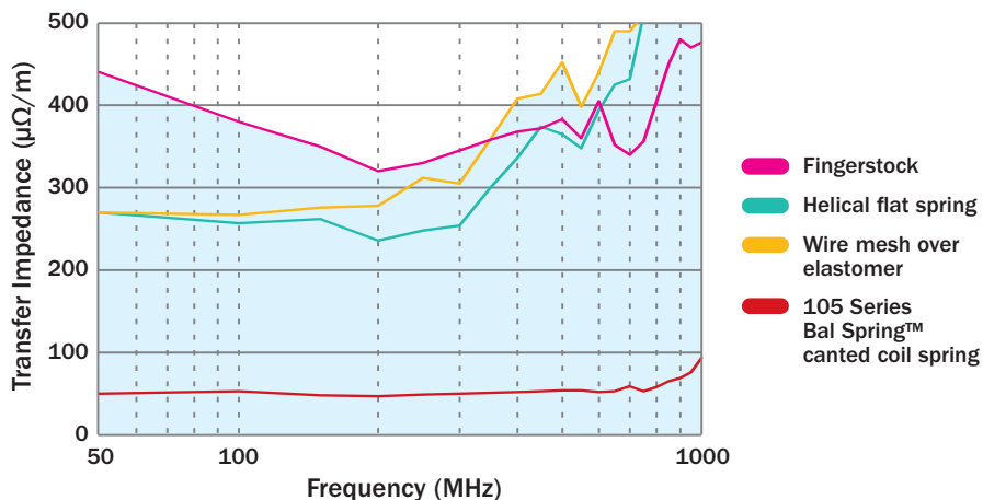
Figure 2. Transfer impedance of canted coil spring vs. other shielding methods.
