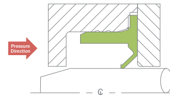
High-speed Flanged Seal
