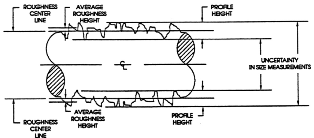
Relationship of Surface Finishes to Dimensional Tolerances FIGURE 5
