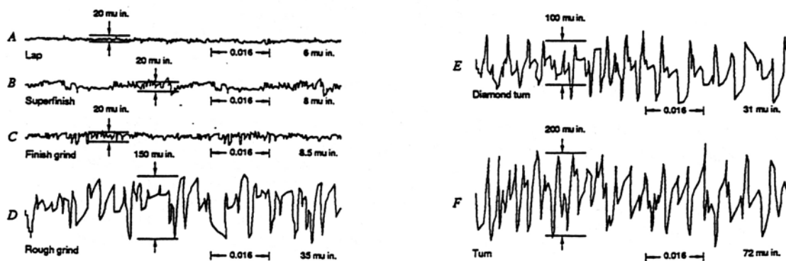
Profile Recordings of Various Machined Surfaces FIGURE 4
