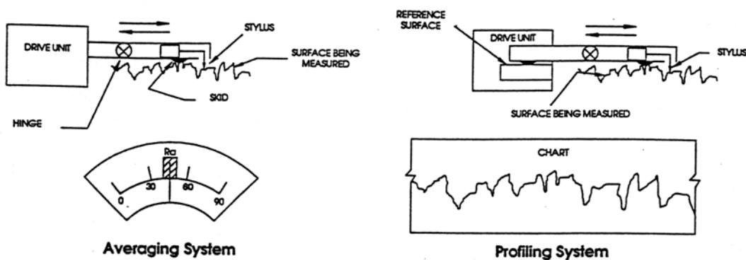
Surface Finish Measuring Instruments FIGURE 3
