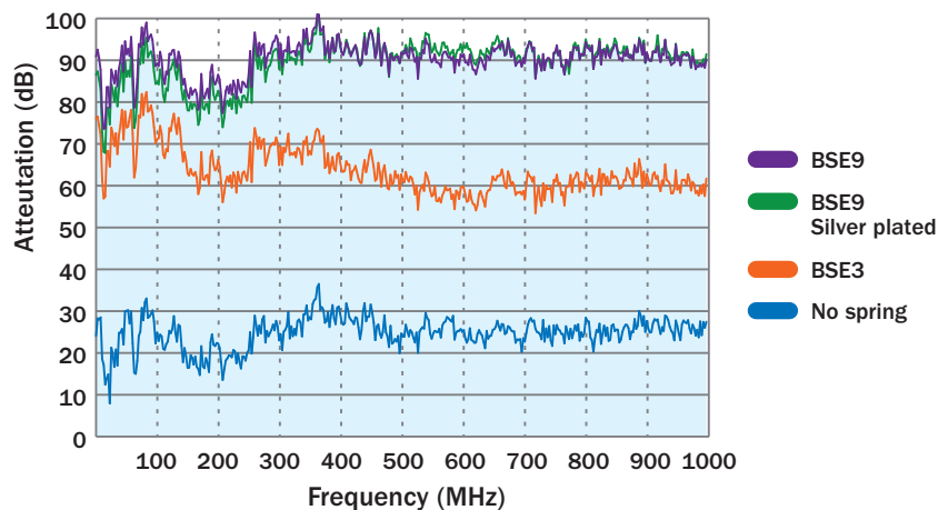
Figure 3. 100 MHz–1 GHz, attenuation vs. frequency.
