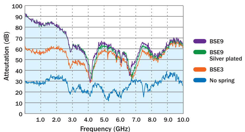
Figure 4. 1–10 GHz, attenuation vs. frequency.
