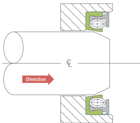
Shaft assembly
