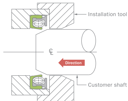
Shaft assembly using installation tool
