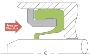
High-speed Seal
