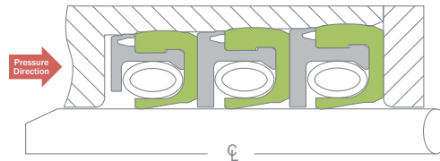
Multi-sealing, Medium-speed, Medium-pressure
