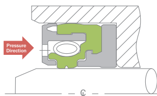
Anti-blowout Seal
