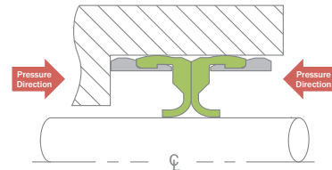
Multi-sealing, High-speed, Low-pressure Seal
