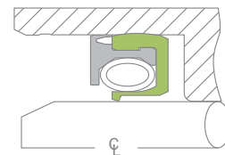
High-speed Seal
