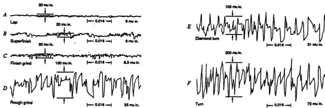
Profile Recordings of Various Machined Surfaces FIGURE 4
