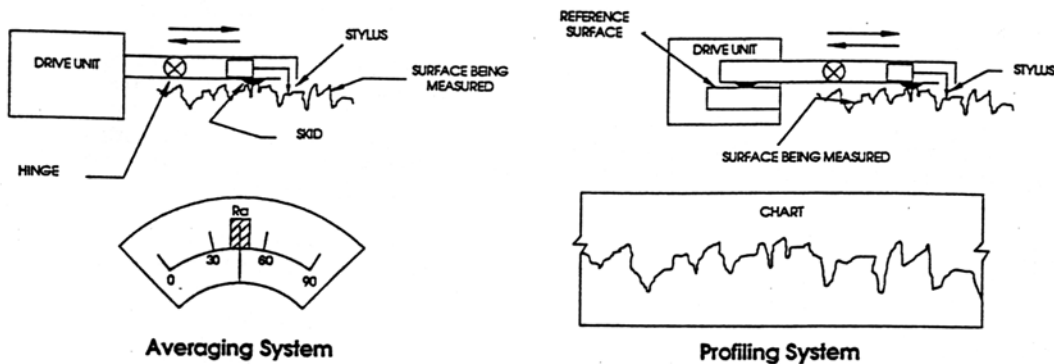
Surface Finish Measuring Instruments FIGURE 3
