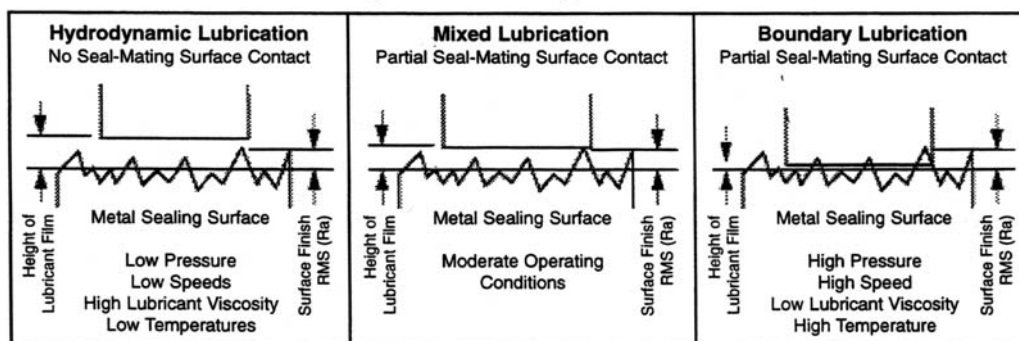
Figure 1: Lubricating Conditions
